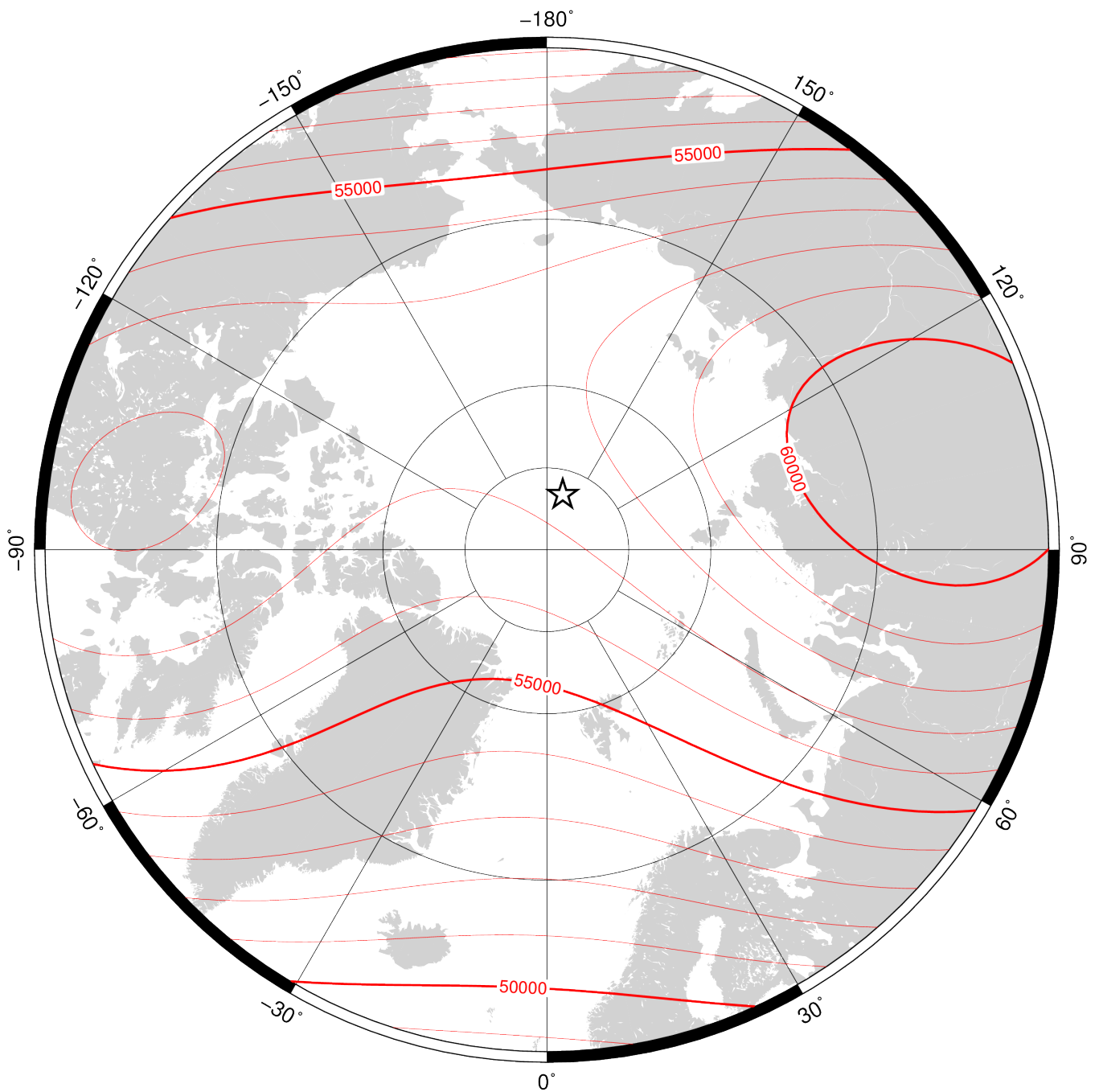
Vertical component ( Z ) in region of north pole at 2020.0 from the World Magnetic Model (WMM2020). Contour interval is 1000 nT, white star is location of a magnetic pole and projection is Polar Stereographic. Credit: British Geological Survey (UK Research and Innovation).
