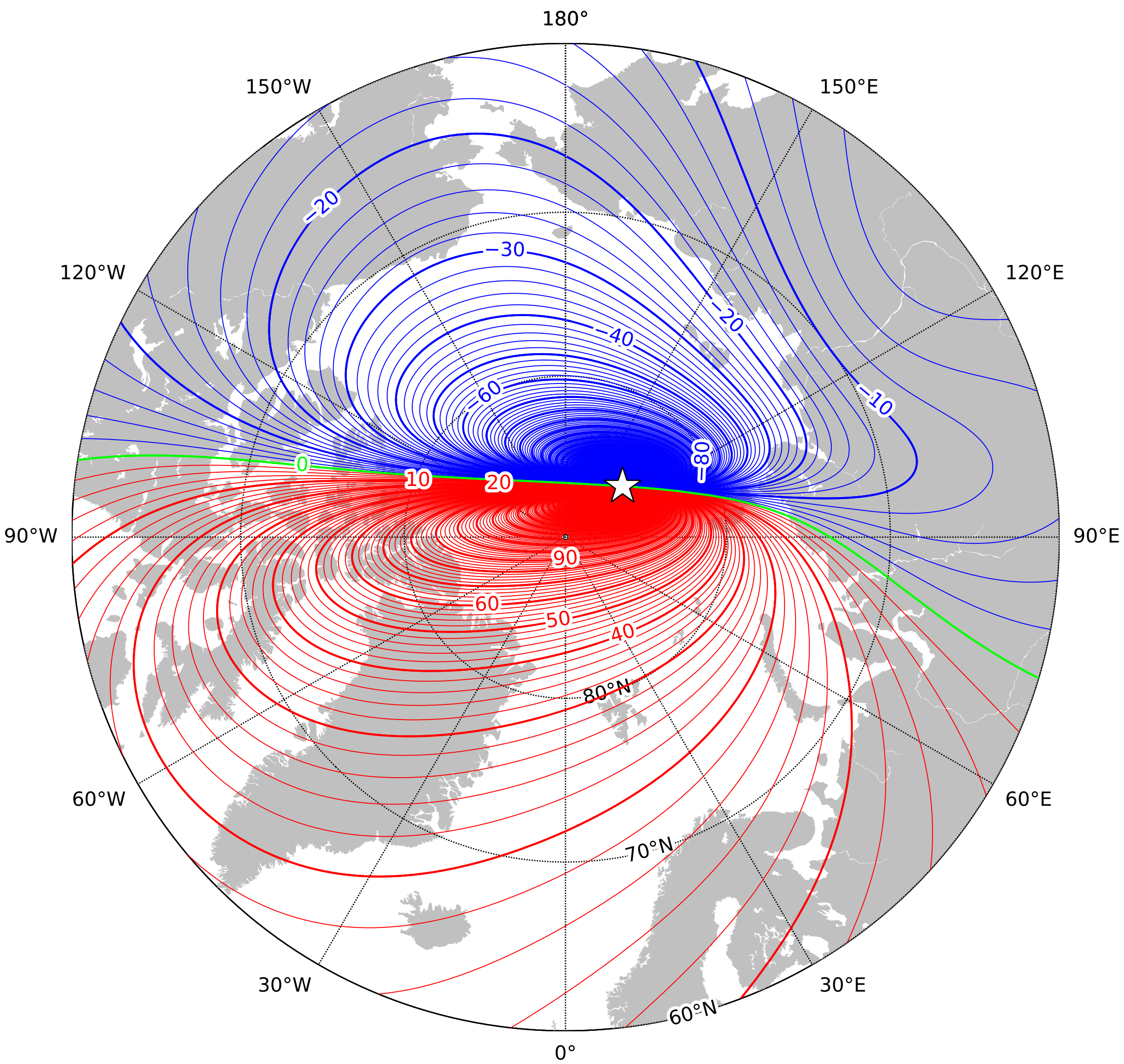
Annual rate of change of declination in the region of the north pole at 2027.5 from the World Magnetic Model (WMM) 2025. Red - positive (easterly) change, blue - negative (westerly) change, green - zero change. Contour interval is 2'/year, white star is the location of a magnetic pole and the projection is Polar Stereographic. This is an example of an isoporic chart. British Geological Survey © UKRI 2024
