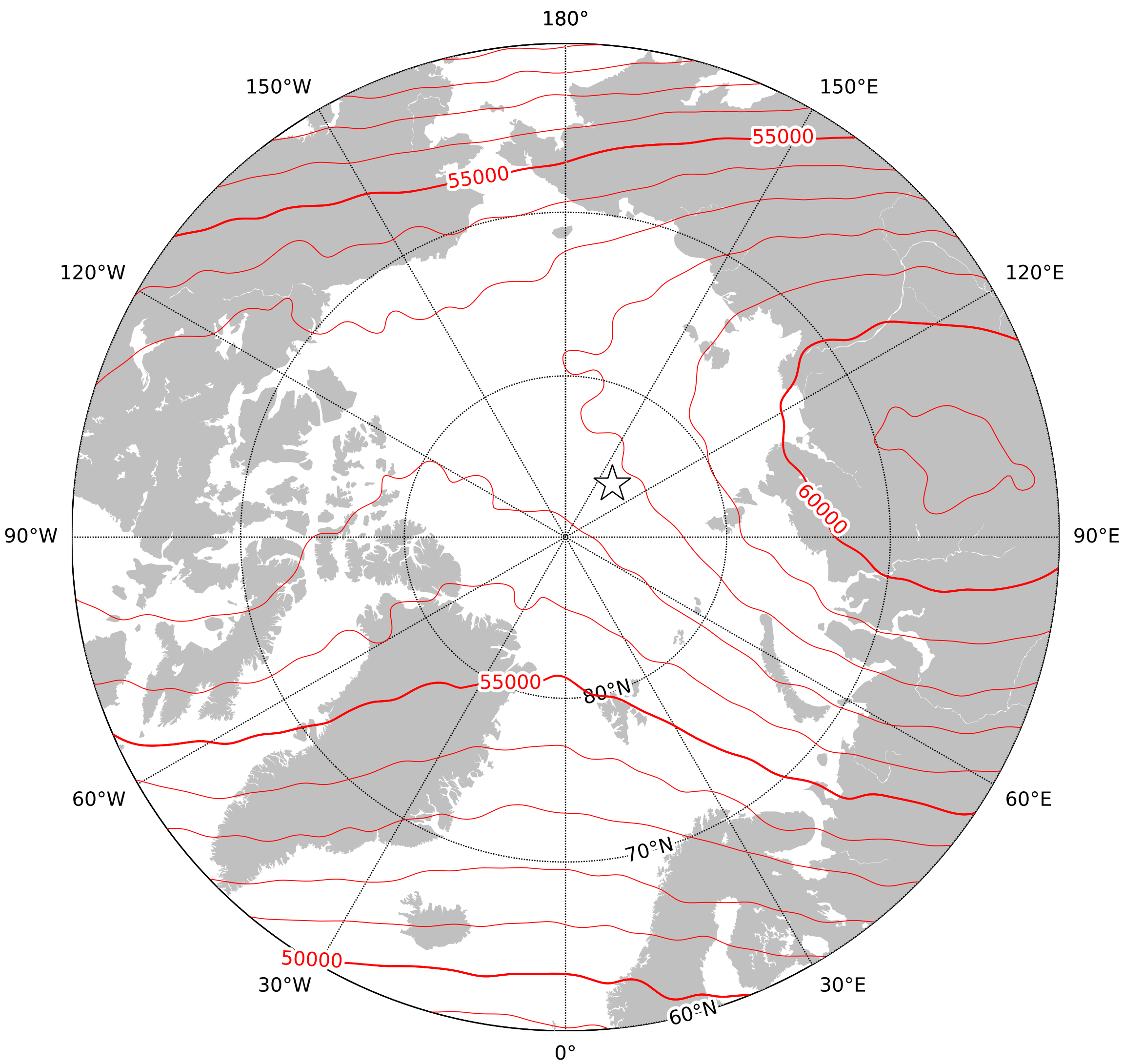
Downward component (Z) in the region of the north pole at 2025.0 from the World Magnetic Model - High Resolution (WMMHR) 2025. Red - positive (down), blue - negative (up), green - zero. Contour interval is 1000nT, white star is the location of a magnetic pole and the projection is Polar Stereographic. This is an example of an isodynamic chart.
