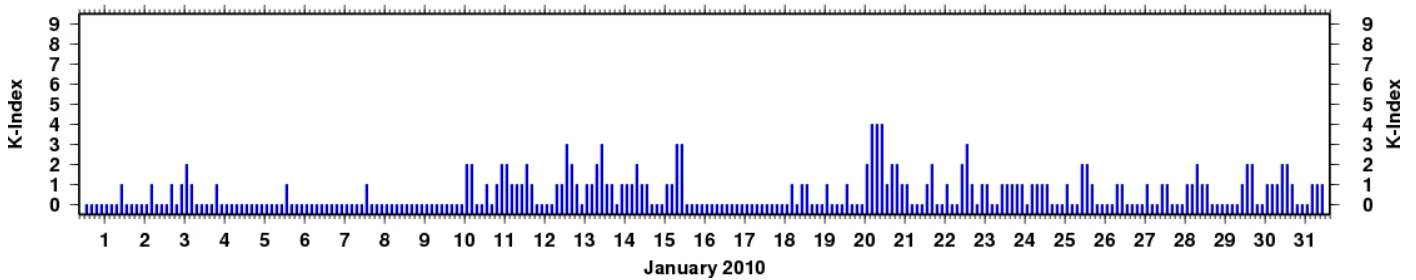
Eskdalemuir Observatory 3-Hourly K-Indices
