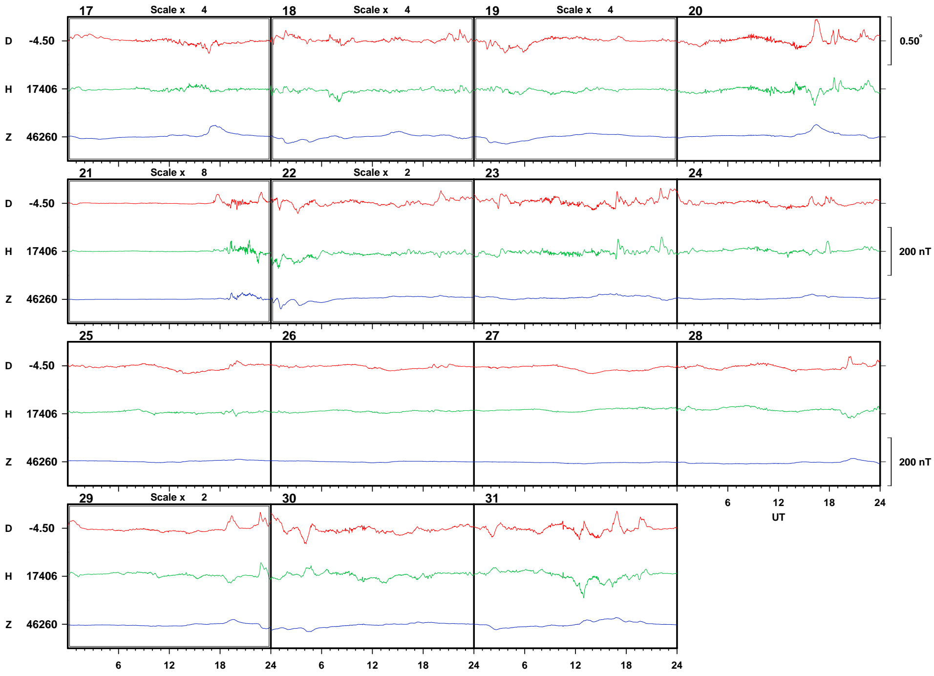
Eskdalemuir January 2005
